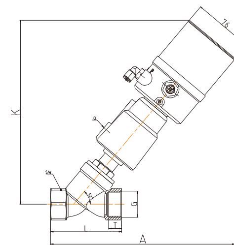
Threaded connection
