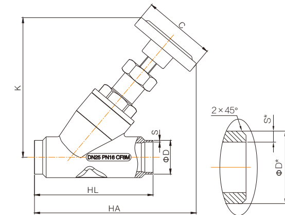
Welded connection
