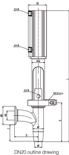
DN20 outline drawing
