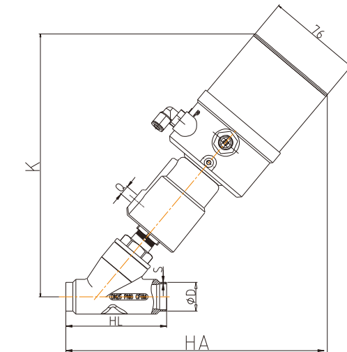
Welded connection
