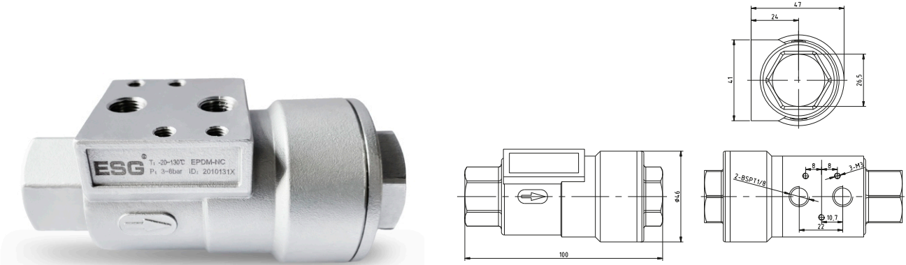
205 Series Pneumatic High-pressure Shuttle Valve
