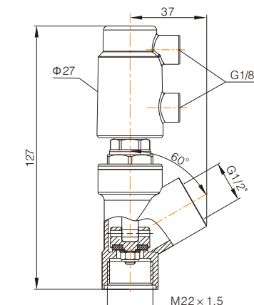
1AB Series Pipe-less Filling Valve
