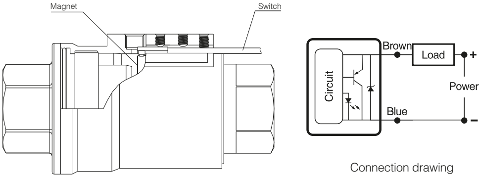
Connection drawing
