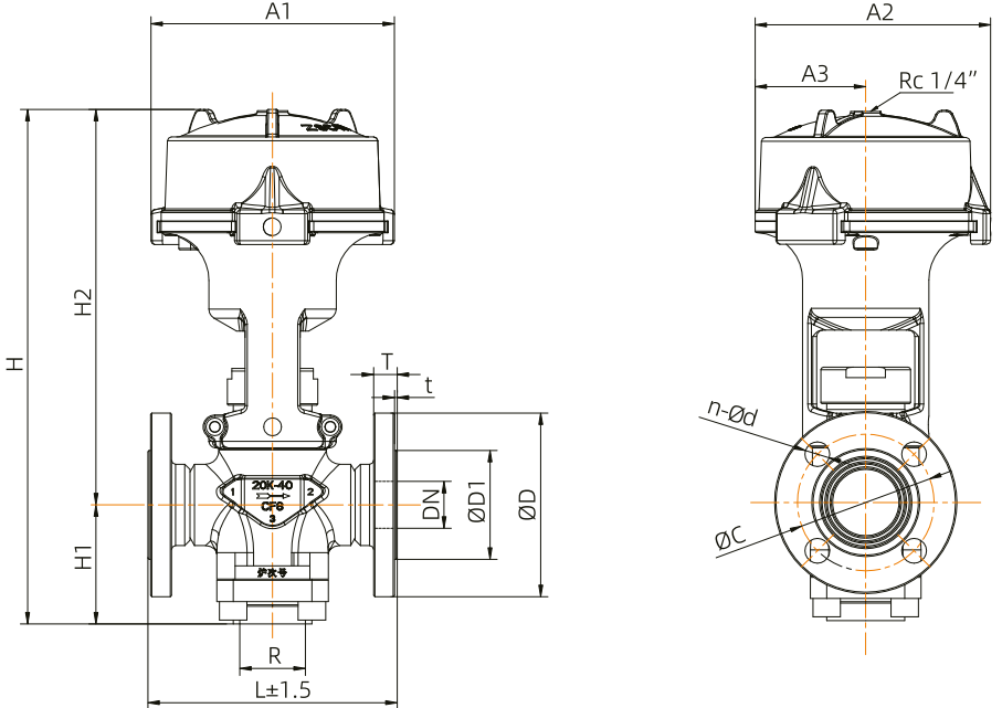
Single Acting Normally Closed, 3-way, Flange
