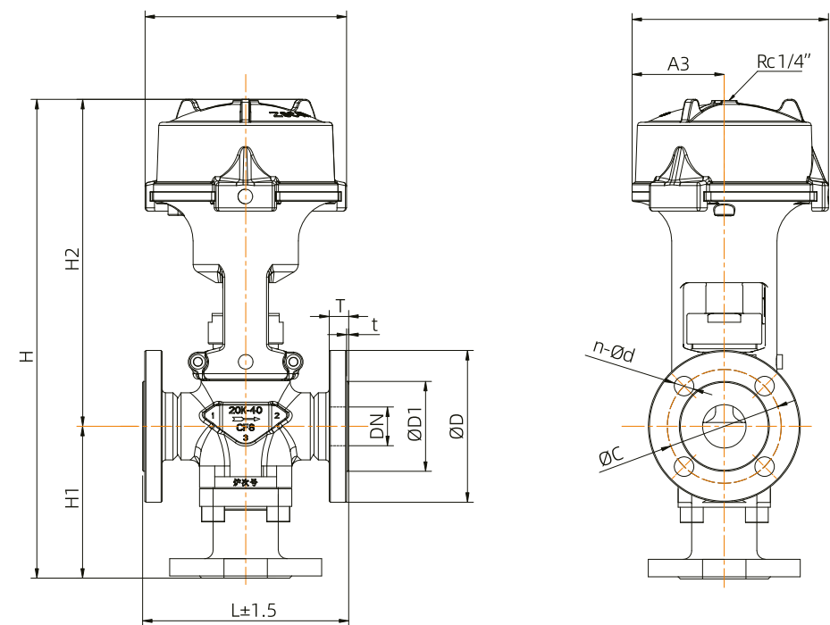
Single Acting Normally Closed, 3-way, Flange
