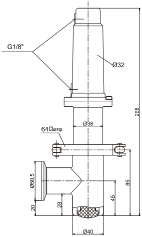
DN25 outline drawing
