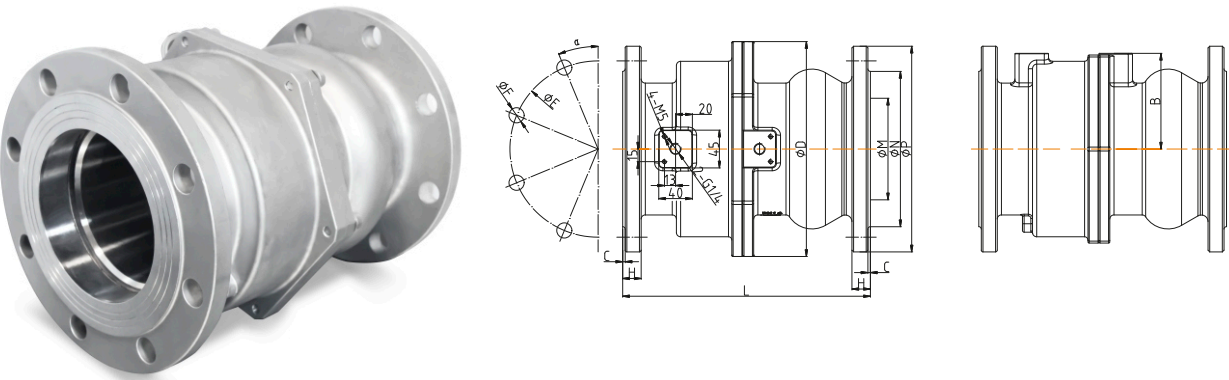
204 Series Flanged Shuttle Valve
