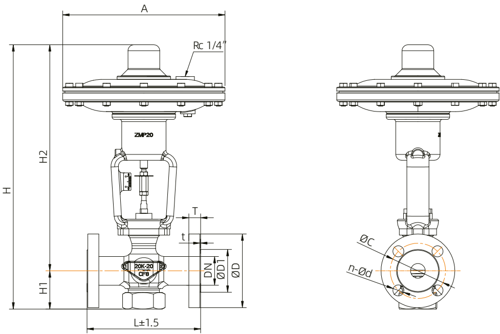
Normally Closed, 2-way, Flange
