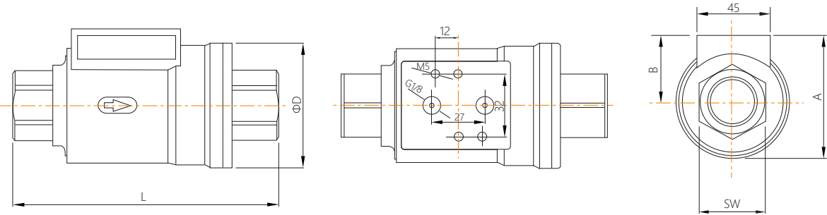
Main Dimension (Threaded connection)
