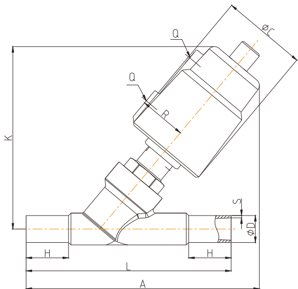
Welded Connection
