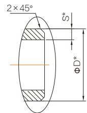
Chamfer
