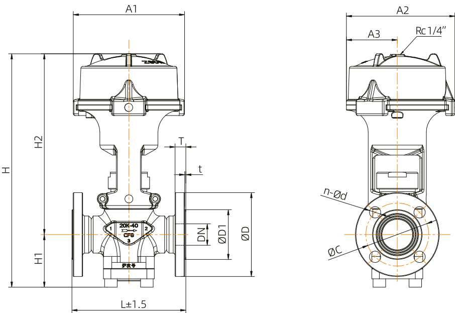
Single Acting Normally Closed, 2-way, Flange
