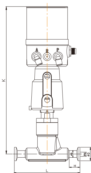
Tri-clamp connection
