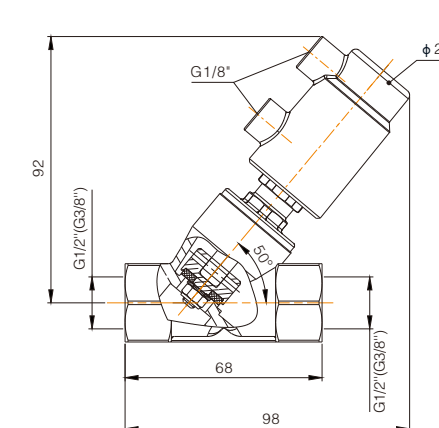
1AA Series 27mm Actuator Pipe-less Filling Valve
